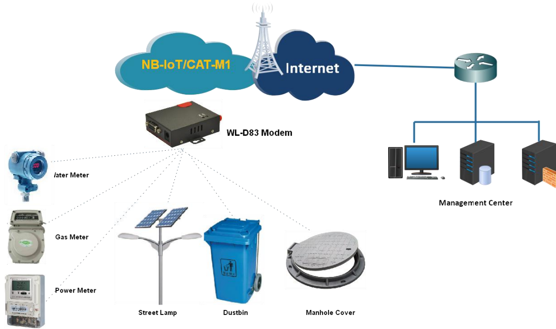
Figure 1-1 Network Topology
