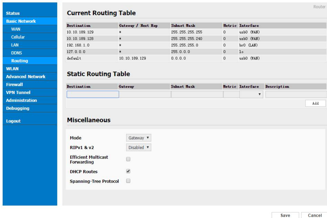
Figure 3-5 Routing Setting
