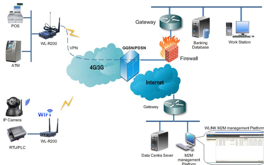
Figure 1-1 Network Topology
